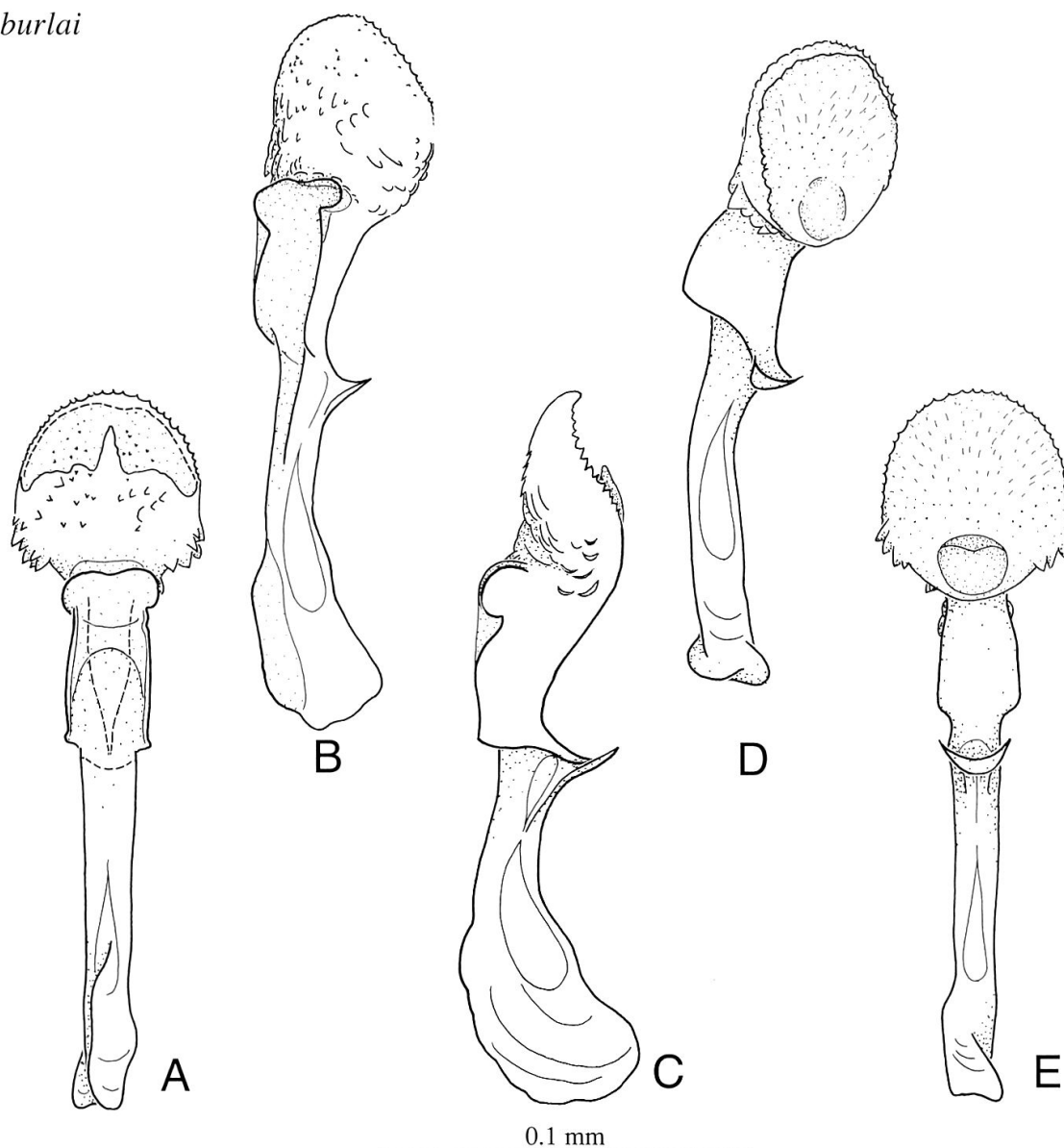
Fig. 9. Paraliodorosophila burlai sp. nov., male holotype. A–E, aedeagus+aedeagal apodeme, several views from dorsal through ventral.
