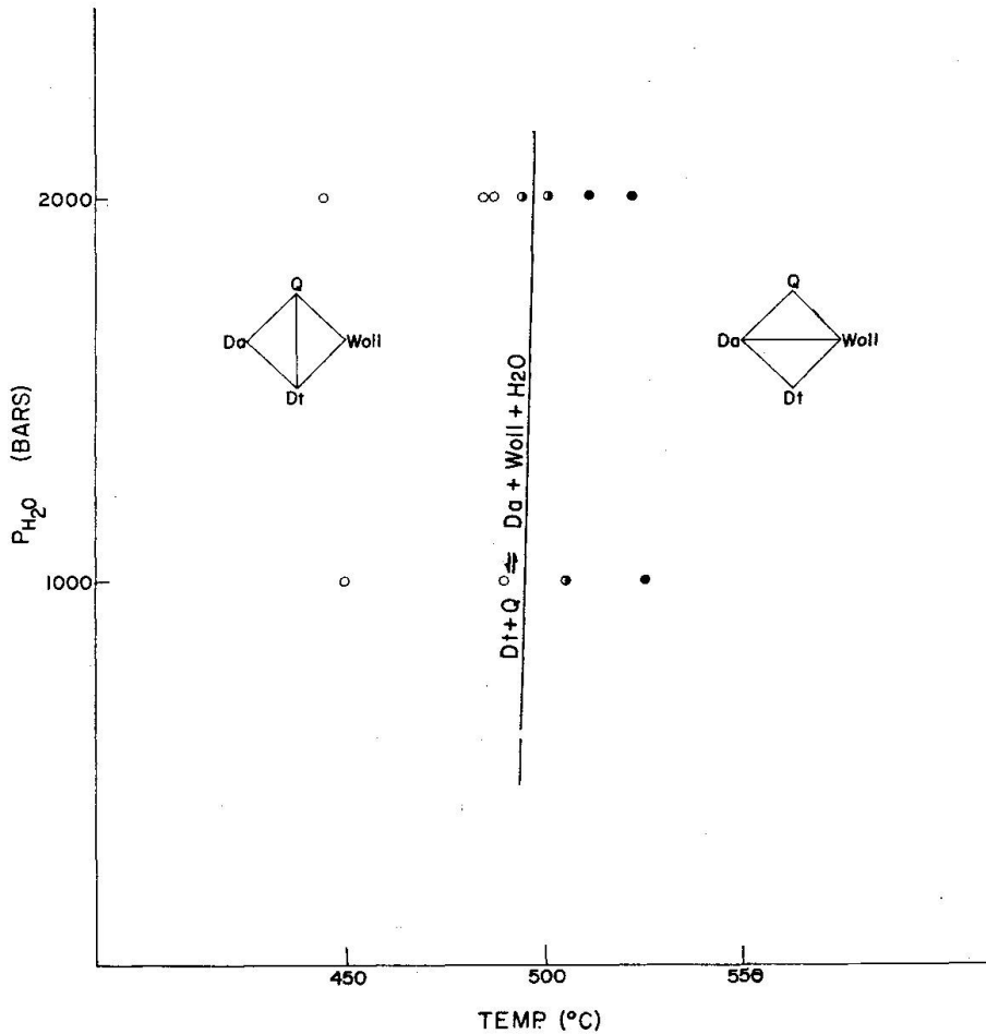
Fig. 5. P_{\text{H}_2\text{O}}\text{-}T diagram for the reaction datolite + quartz \rightleftharpoons danburite + wollastonite + \text{H}_2\text{O} . Da: danburite; Dt: datolite; Woll: wollastonite; Q: quartz.
