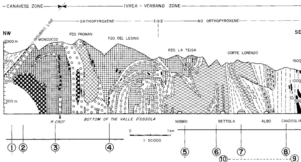
Fig. 1. Profile through the Ivrea-Verbano Zone on eastern side of the Valle d'Ossola, simplified after SCHMID (1967, table X), with positions of the observation points corresponding to this profile (no. 1—4, 9—10 on the western side, no. 5—8 on the eastern side of the Valle d'Ossola). Legend in Fig. 2.
