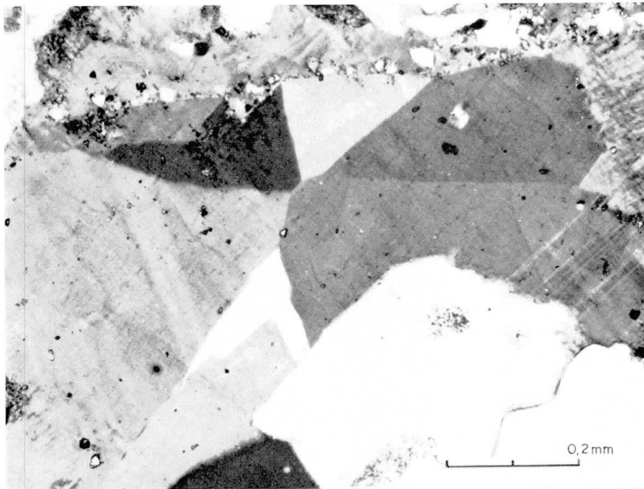
Fig. 4. Tridymite. Crossed polars. Composite crystal of irregular outline. Additional internal division can be seen in two sectors (S, almost white and NW, dark); in one sector (E) there is furthermore a polysynthetic lamellation.
