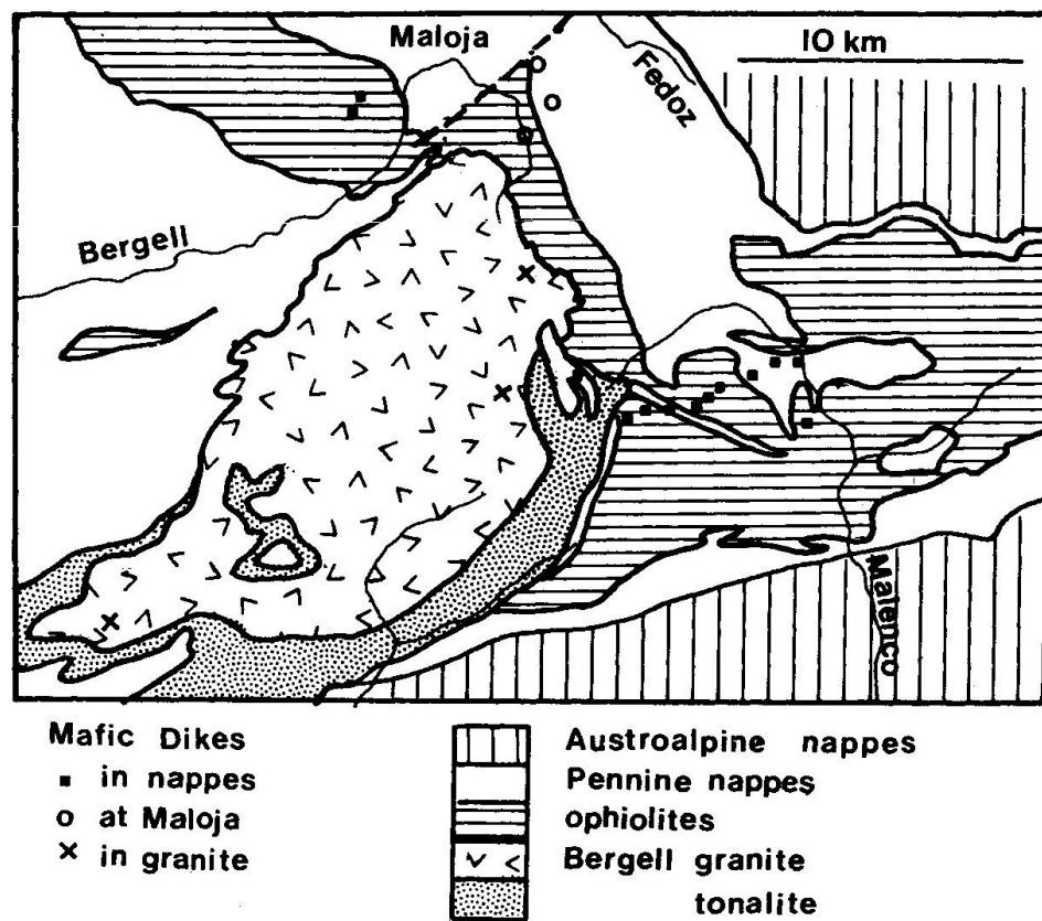
Fig. 1 Tectonic sketch of the Bergell Alps indicating localities of andesitic and gabbroic dikes.
