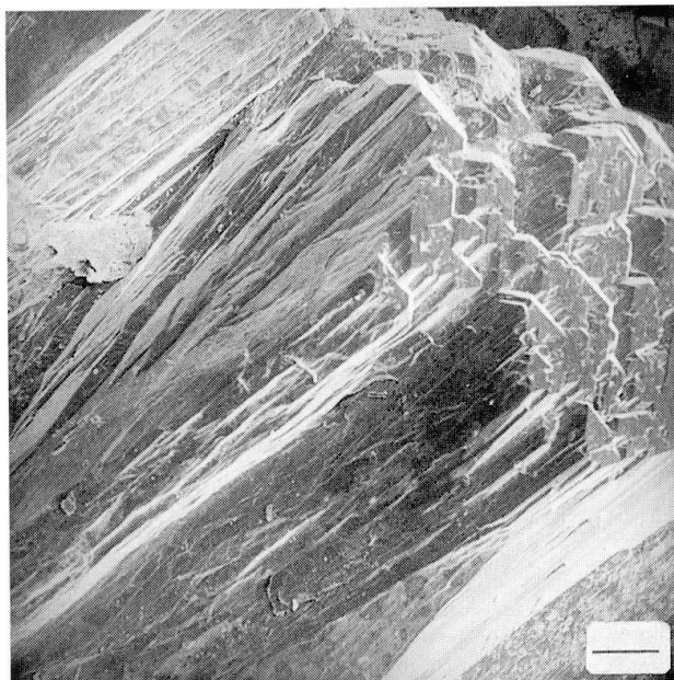
Fig. 2 Scanning-electron microphotograph of Vathi Sr-bearing stilbite. Bar scale = 100 \mu m.
