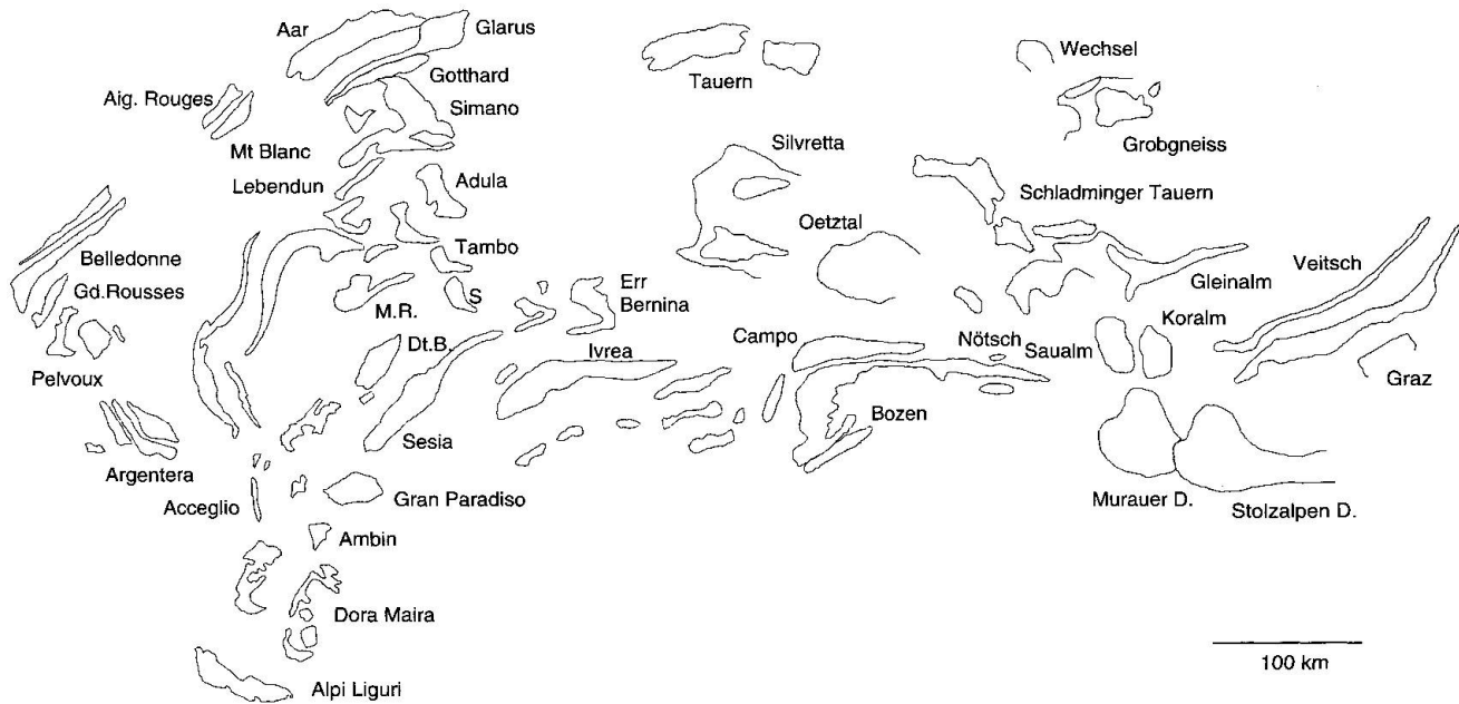
Fig. 2 Pre-Mesozoic palinspastic reconstruction of the pre-Mesozoic basement in the Alps after figure 2 in VON RAUMER and NEUBAUER (1993) and based on the reconstructions of NEUBAUER (1988); DE GRACIANSKY (1993); PFIFFNER (1993); RATSCHBACHER and FRISCH (1993), with indication of names of the different units.
