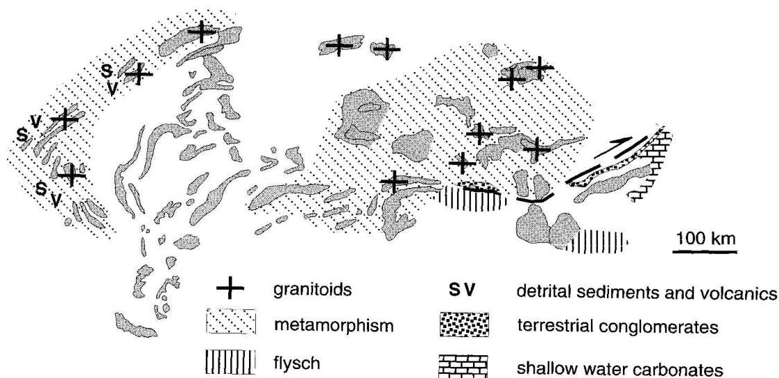
Fig. 3 Pre-Mesozoic basement in the Alps (approximate Late Variscan configuration, see Fig. 2) and distribution of tectonostratigraphic events for distinct time periods.
