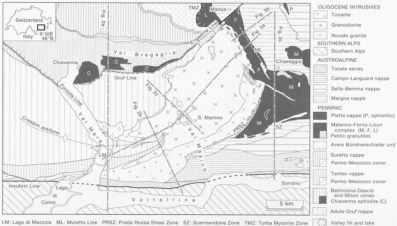
Fig. 1 Tectonic map of the Bergell pluton and surrounding tectonic units. Traces of profiles presented in figures 2 and 3 are indicated.
