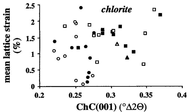
Fig. 9 Apparent mean lattice strain versus chlorite crystallinity. For legend see the caption of figure 5.
