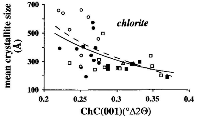
Fig. 8 Apparent mean crystallite size of chlorite as a function of chlorite crystallinity. For legend see the caption of figure 5.
