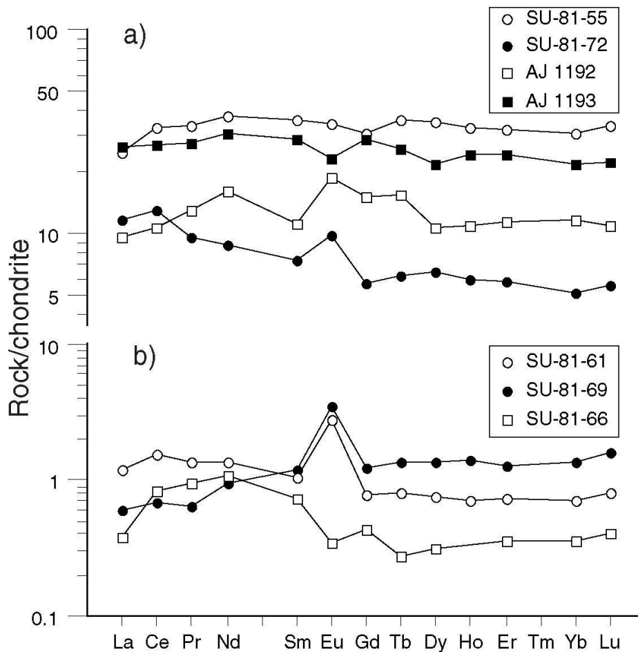
Fig. 3 Rare earth element variation diagram for: (a) amphibolites; (b) hornblende-felses and serpentinite.
