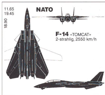
F-14 Tomcat
