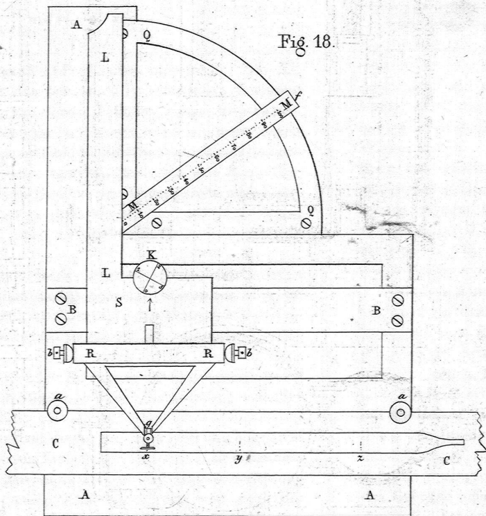
Charles' Pendelwage.
