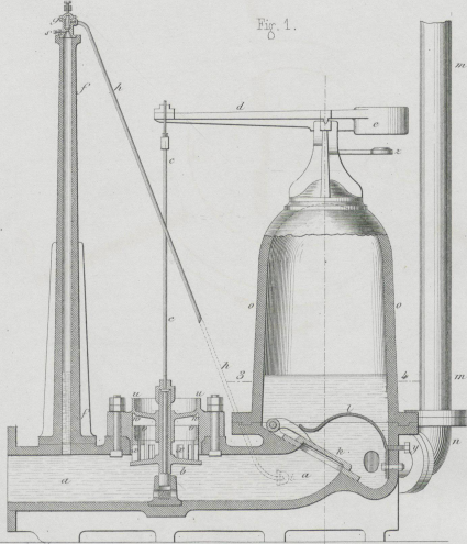
Bollee's Stosshaber.
