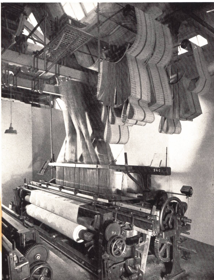
Jacquard loom for linen-weaving.
