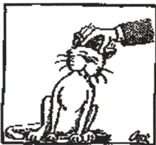
Theoretician's Cat
