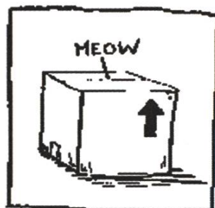
Experimentalist's Cat
