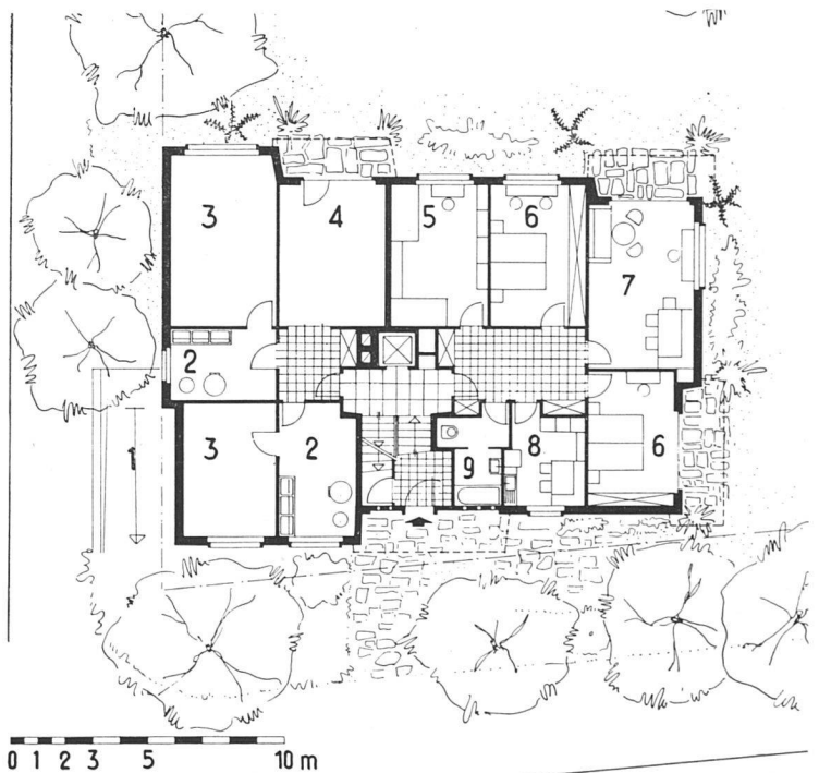
Erdgeschoß 1:300 | Rez-de-chaussée | Ground floor
