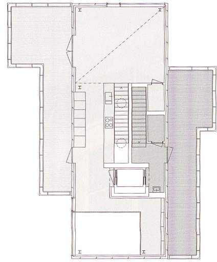
Attikageschoss
