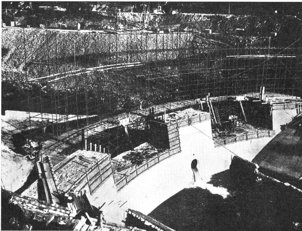
Staumauer Couesque in Frioplast-Beton
