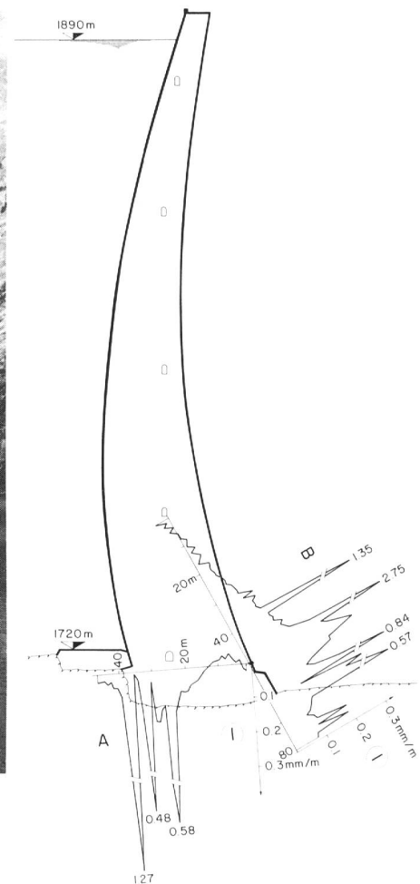
Figure 5. Kölnbrein, arch dam, block 18. Sliding micrometer, measuring results. A Strain distribution due to reservoir filling, extension strain. B Strain distribution due to reservoir emptying, extension strain.
